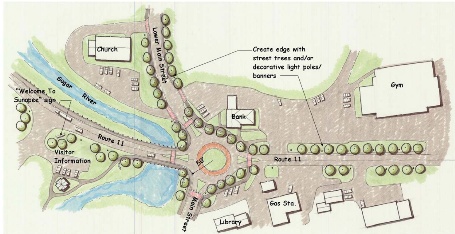
Sunapee, New Hampshire Roundabout Concept Plan
